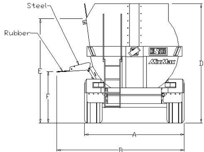
Feedout chute details
